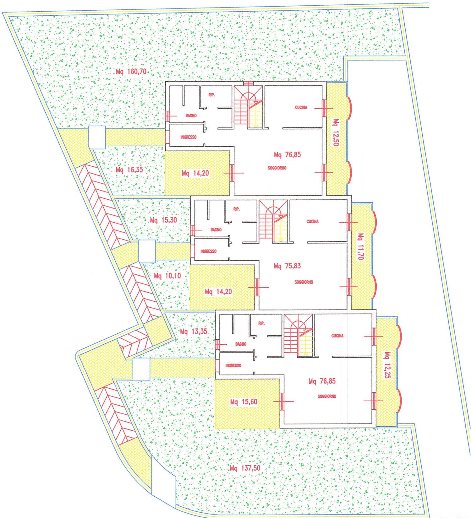
PIANO TERRA
